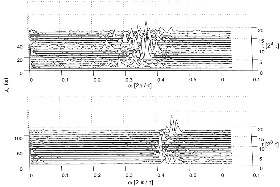
Figure 4: The window-time behavior of the first memory function power spectra \mu_1(\omega) for young and elderly people. On certain frequencies the dynamic peaks are distinctly visible in both power spectra. These peaks are connected with respiratory arrhythmia. These peaks are shifted towards higher frequencies for elderly people. It confirms the conclusion made as a result of the analysis of the previous figure.
